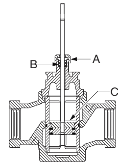
Repair Parts, V-5464
