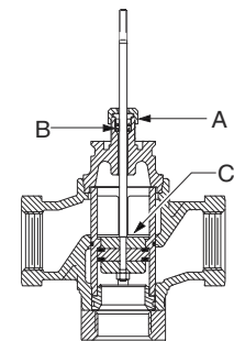
Repair Parts, V-5844
