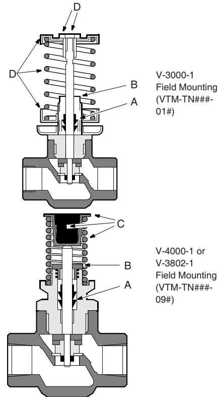
Repair Parts, VT Series Valves
