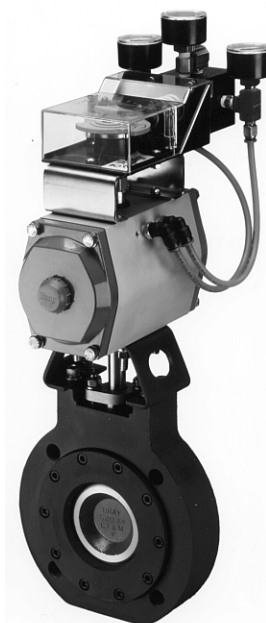
Two-Way High Performance Valve with Industrial-Grade, Spring Return, V-919x Series High Pressure Pneumatic Actuator
