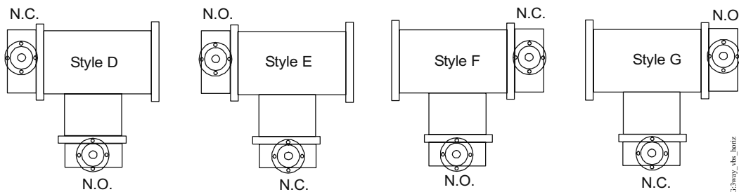
Three-Way Valve Body Styles
