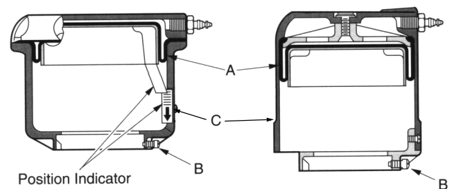
Repair Parts, V-3000 Actuator
