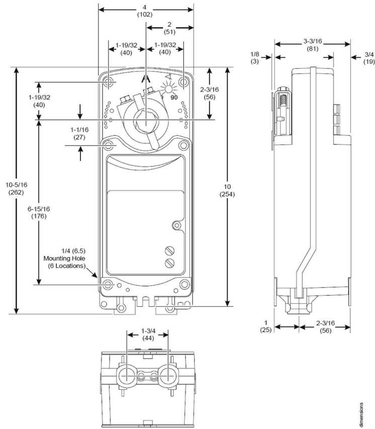
M9210-xxx-3 Series Electric Spring Return Actuator Dimensions, in. (mm)
