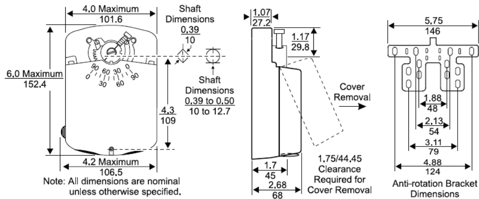
Dimensions, in./mm
